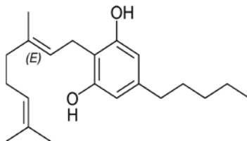
Fig. 9: Cannabigerol
