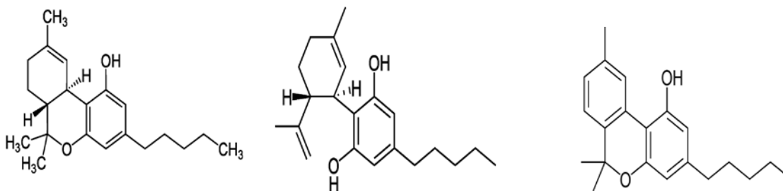
Fig.5: Tetrahydrocannabinol(THC) Fig.6: Cannabidiol (CBD) Fig. 7: Cannabinol (CBN)
