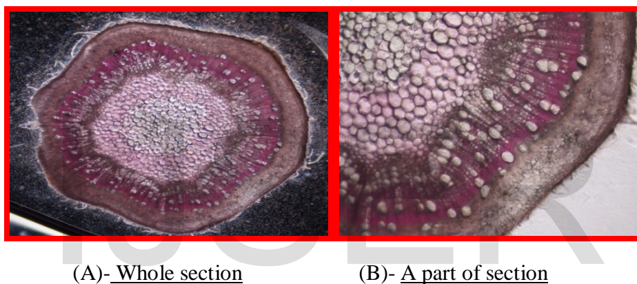
Fig.11 (A & B)-Transverse section of Stem of Cannabis Sativa
