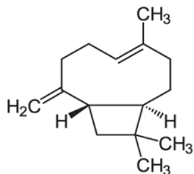
Fig. 8: \beta - Carophyllene
